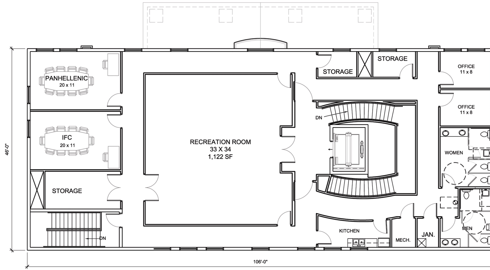
SECOND FLOOR PLAN Schematic
